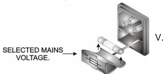
Battery charger ALTAIR WBPC-200 set up to 115 V.
