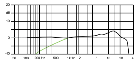
Frequency Response (d:fine™ 4088 and d:fine™ 88)
